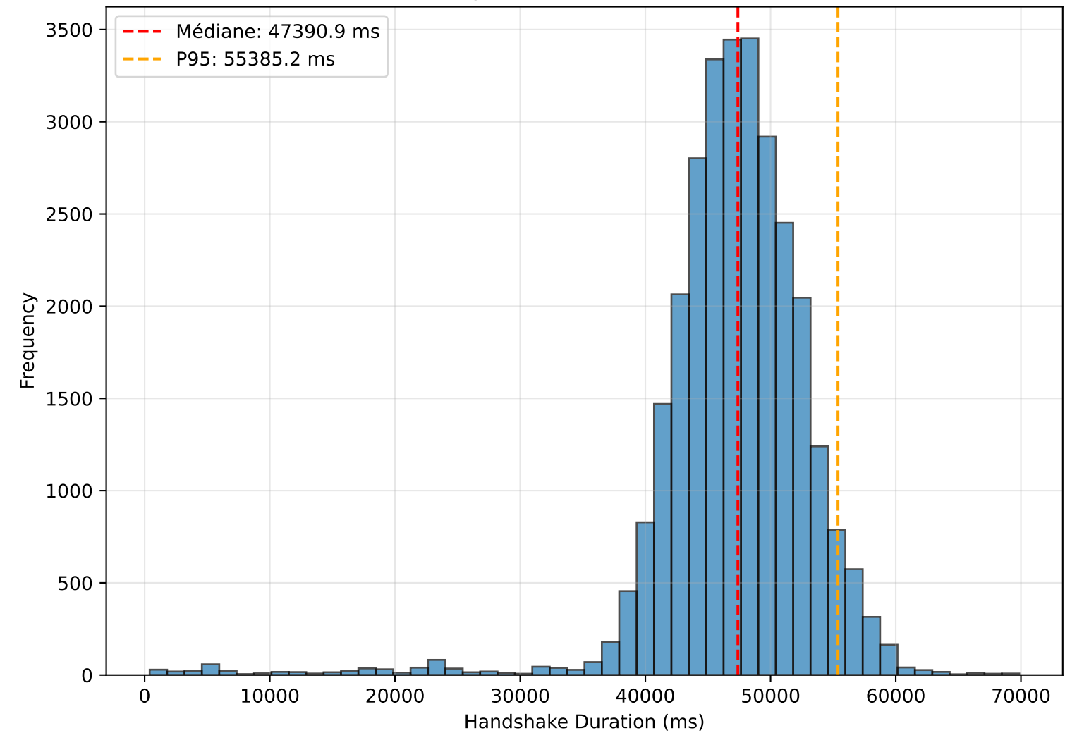
Distribution globale — mldsa65 × mlkem768
