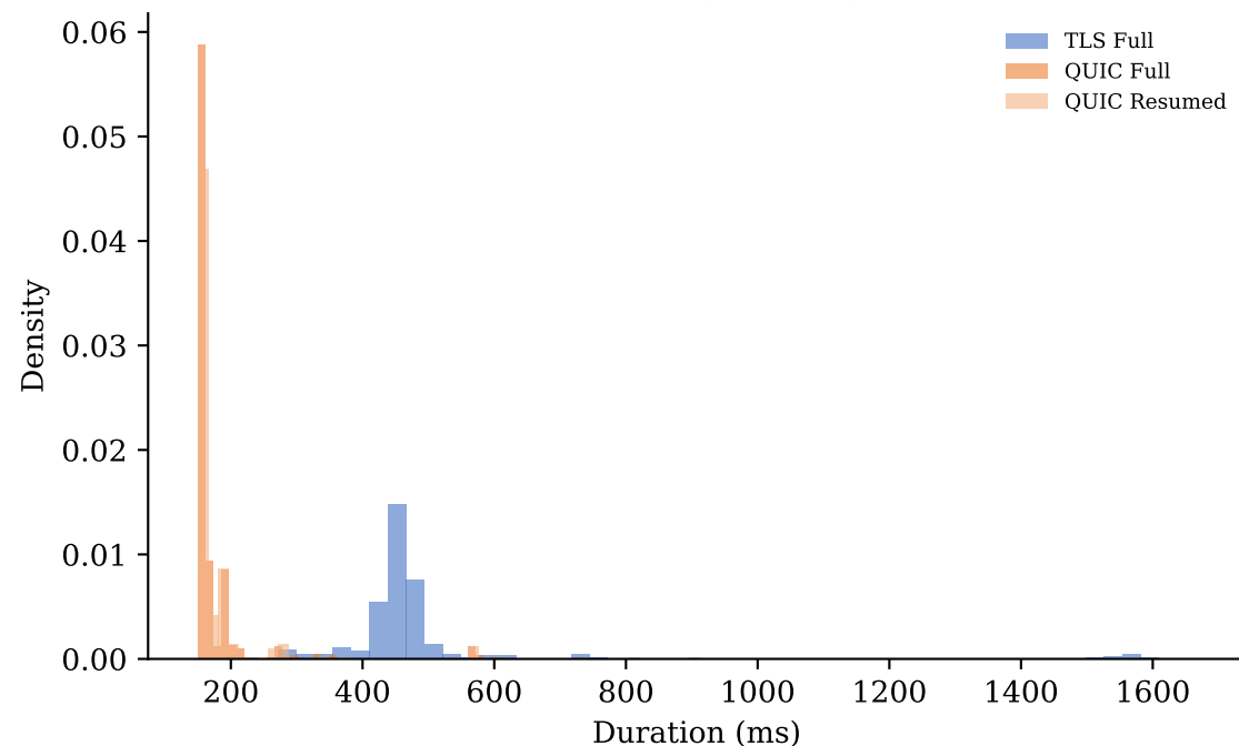
GE Stable
