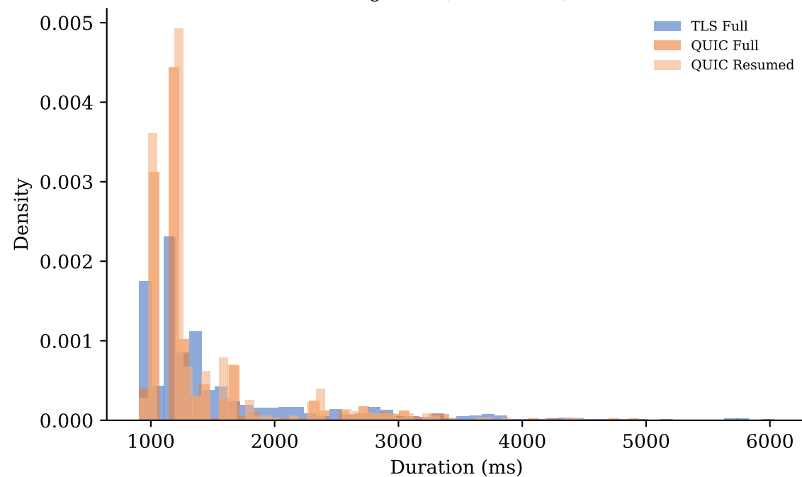
Degraded (200ms/10%)
