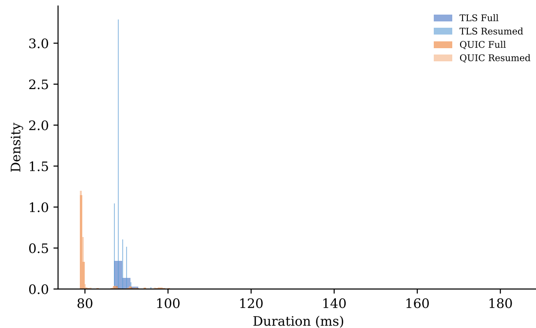
GE Stable
