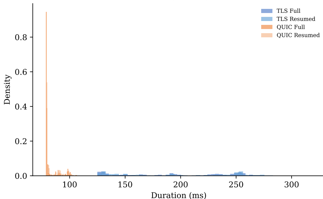
Degraded (200ms/10%)
