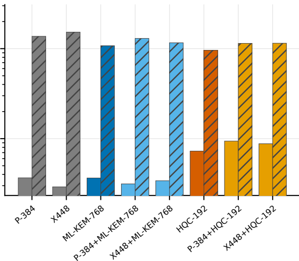
secp384r1 (classical)
