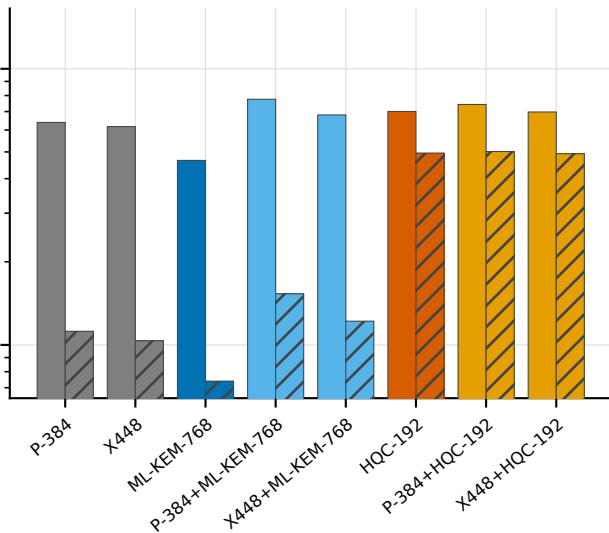
secp384r1 (classical)
