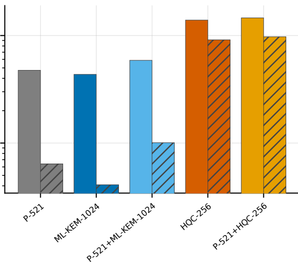
secp521r1 (classical)
