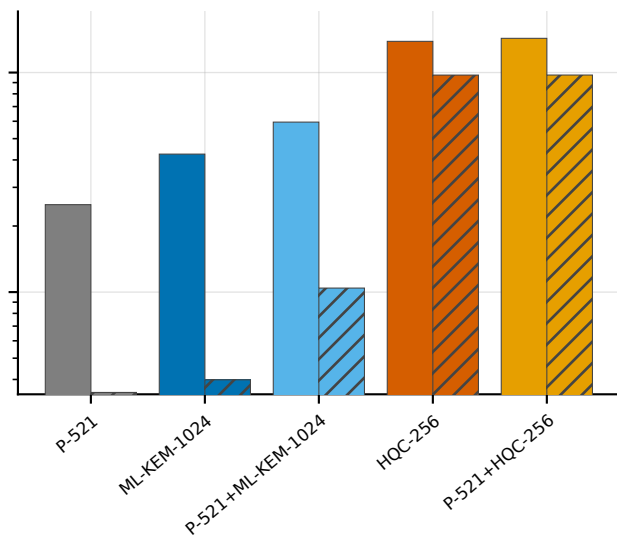
mldsa87 (post-quantum)
