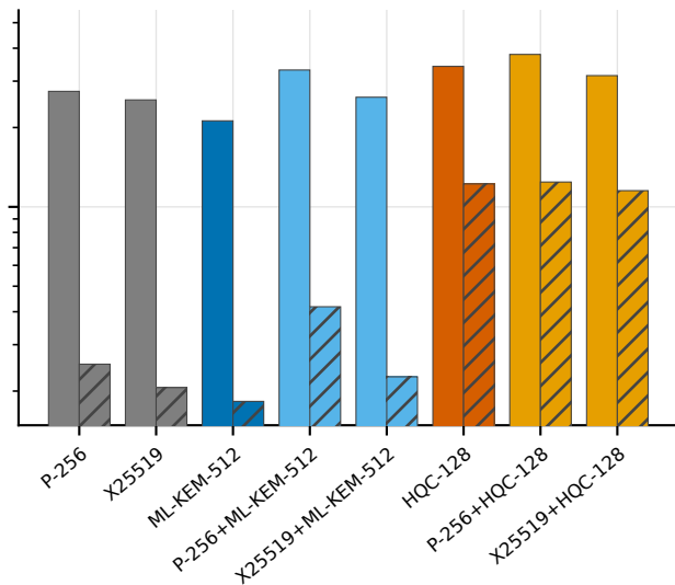
mldsa44 (post-quantum)
