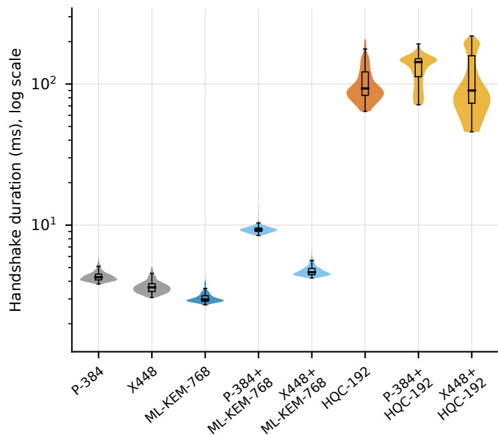
secp384r1 (classical)
