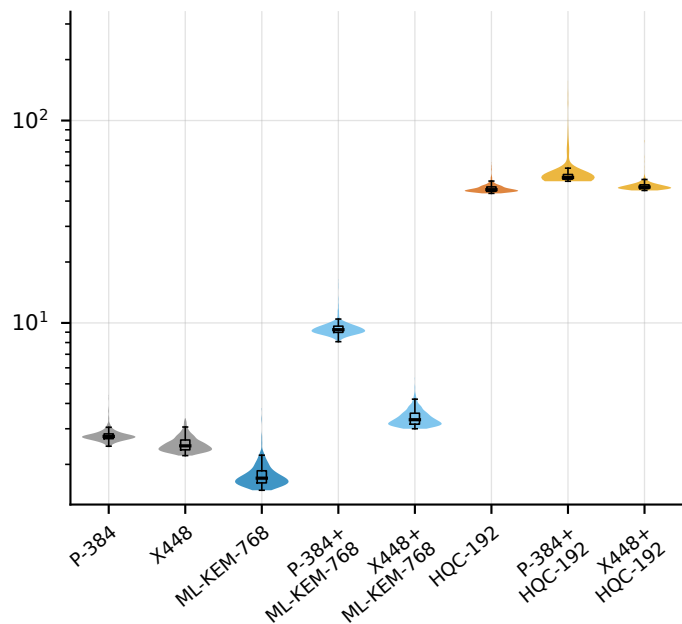
mlds65 (post-quantum)
