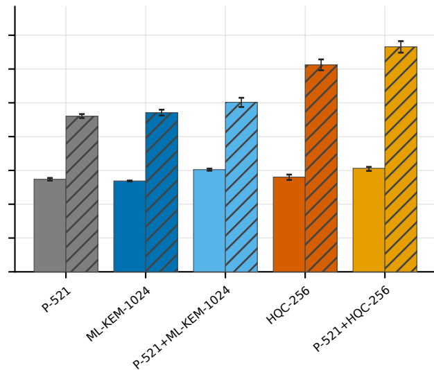
mlDSA87 (post-quantum)
