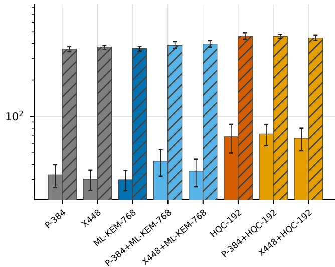
secp384r1 (classical)
