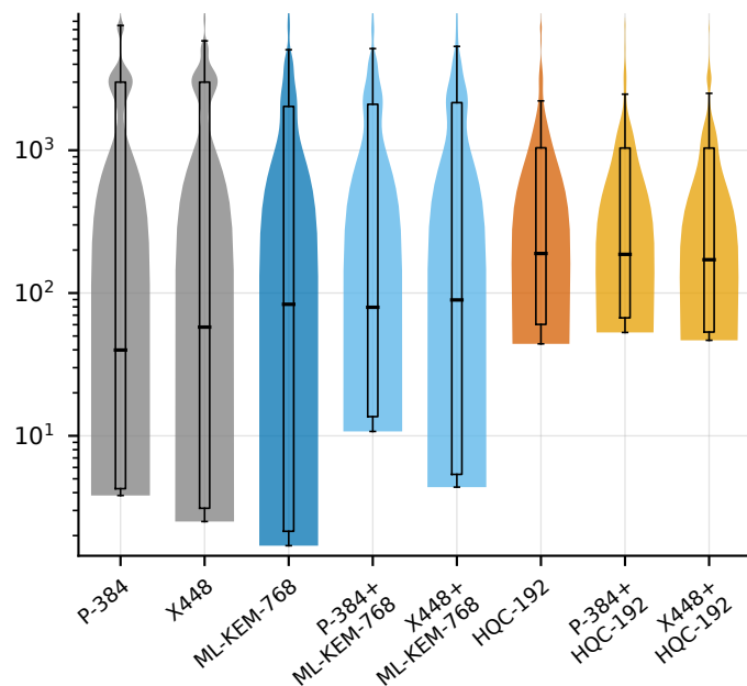
mlds65 (post-quantum)
