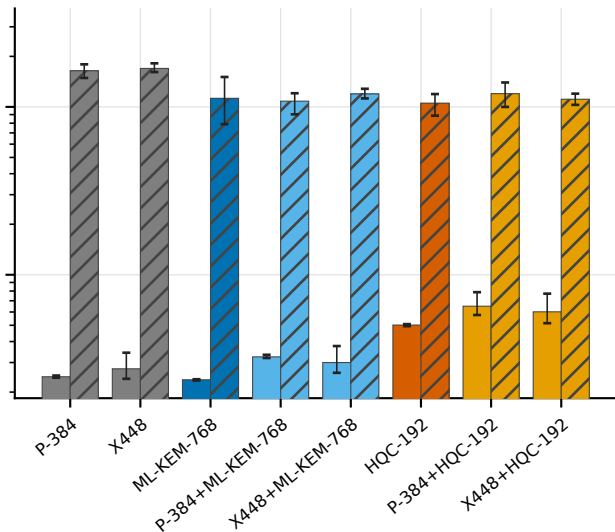
secp384r1 (classical)
