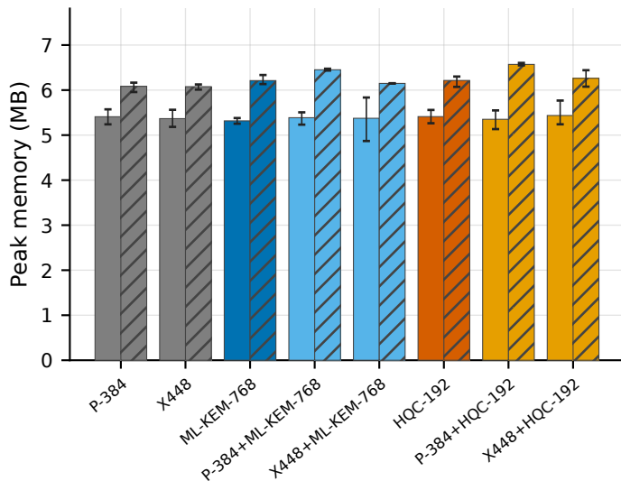
secp384r1 (classical)
