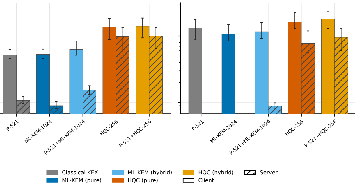
secp521r1 (classical)
