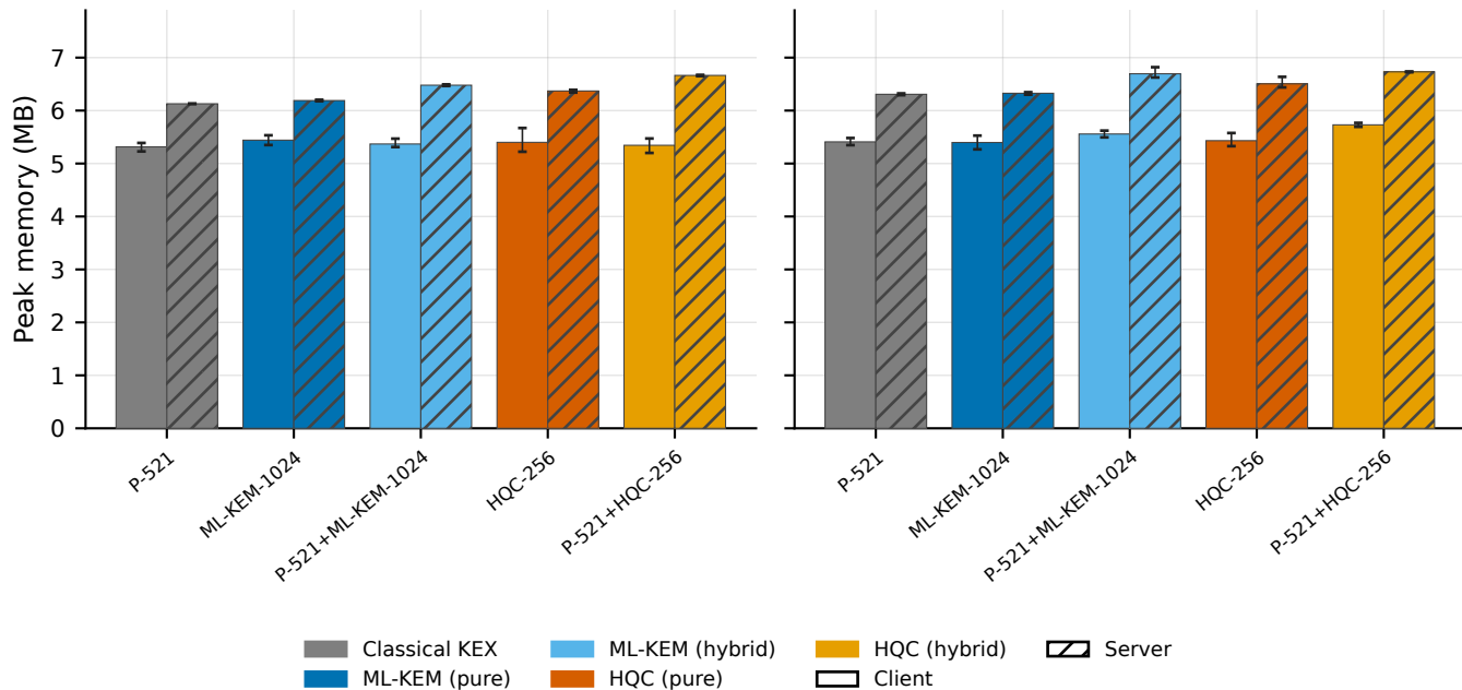
secp521r1 (classical)
