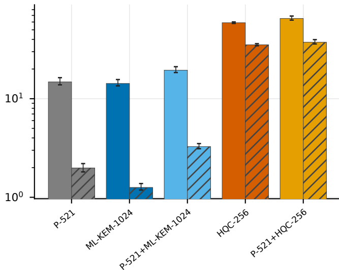
secp521r1 (classical)
