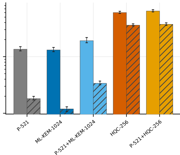
mldsa87 (post-quantum)
