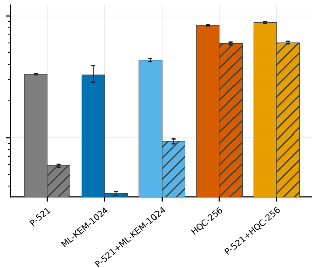
mldsa87 (post-quantum)
