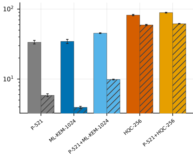
secp521r1 (classical)
