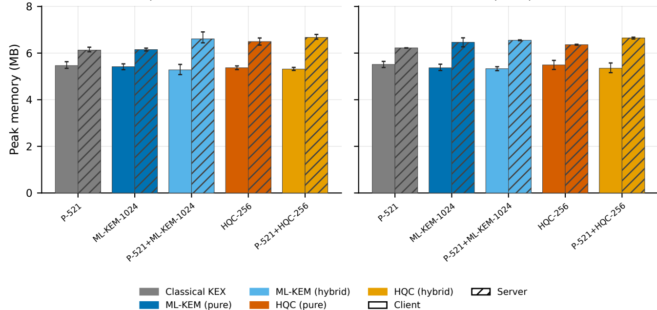
secp521r1 (classical)
