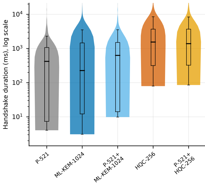
secp521r1 (classical)
