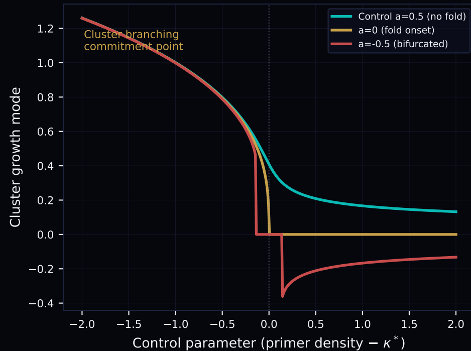
D. Whitney A_1 fold at cluster branching
