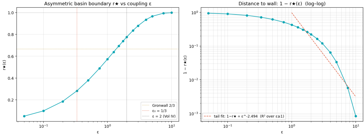
Figure 4: Left: r_\star(\varepsilon) on a log- \varepsilon scale. Markers from DOP853 bisection at 17 values of \varepsilon . The Gronwall threshold \varepsilon_0 = 1/3 and the Vol. IV canonical \varepsilon = 2 are marked. Right: 1 - r_\star(\varepsilon) on log-log axes. The dashed power-law fit on \varepsilon \geq 1 is a poor model; the local slope steepens as \varepsilon grows, indicating super-polynomial decay.
