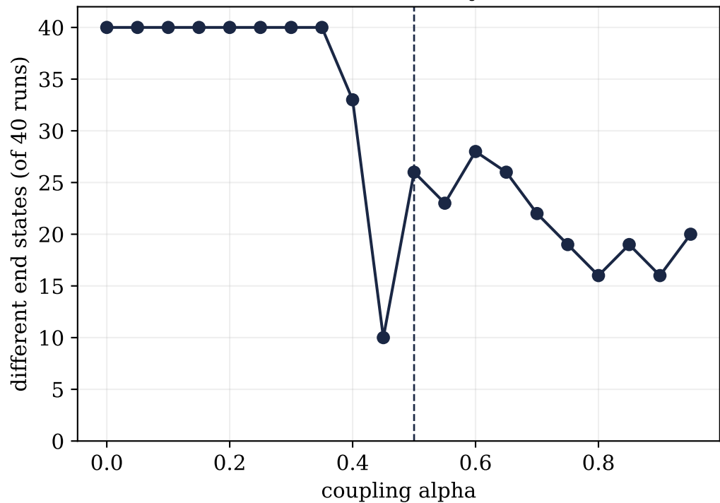
Multistability
