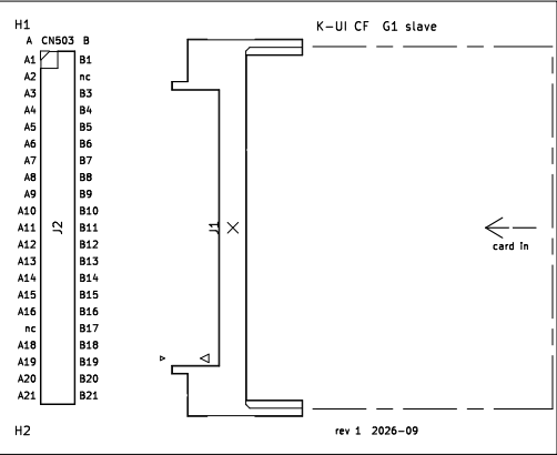
K-UI CF board: fit template (board 66.5 x 54 mm, card slides in from the right)
