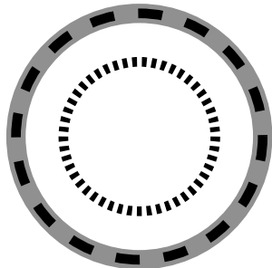
NoConsequence NOC
