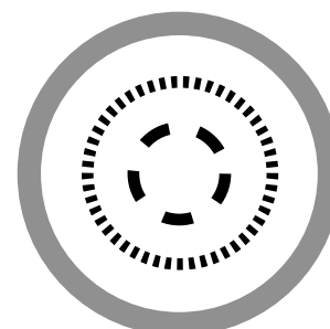
WeakerThm WTH
