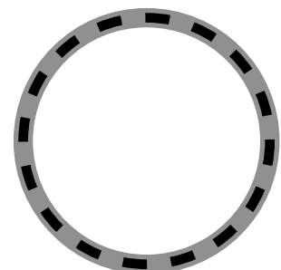
Unsatisfiable UNS
