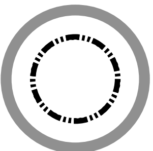
EquivThm ETH
