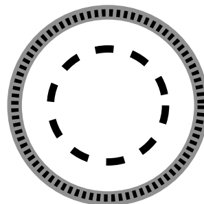
WeakerTautConc WTC
