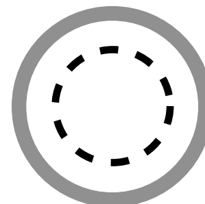
WeakerUnsConc WUC
