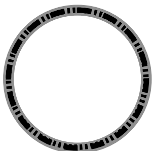
Tautology TAU
