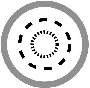
Satisfiable SAT
