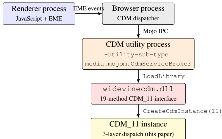
Figura 1: End-to-end Widevine EME dispatch on Chromium-family browsers on Windows. The host browser delegates Encrypted Media Extensions operations through Mojo IPC to a utility process whose sole purpose is to load widevinecdm.dll and expose its CDM_11 interface. This paper studies the dispatch model that sits between the CreateCdmInstance -returned interface and the per-slot handlers inside the library.
