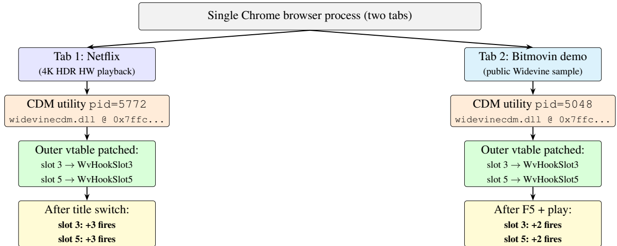
Figura 6: Cross-source experiment. Two tabs of the same Chrome browser play two distinct Widevine-protected sources, each one served by its own CDM utility process. Identical hooks confirm identical session-management slot reachability.
