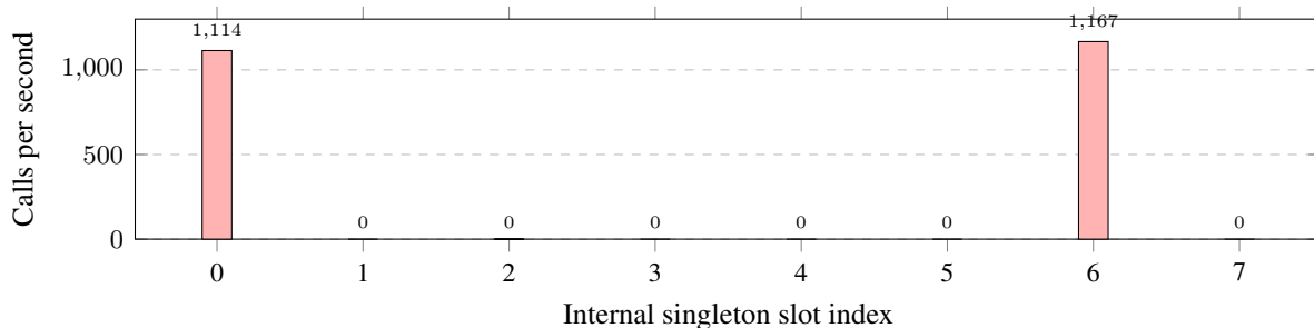
Figura 5: Activity profile of the internal singleton dispatch table at .data + 0x1588b48 during steady-state Netflix 4K HDR playback.
