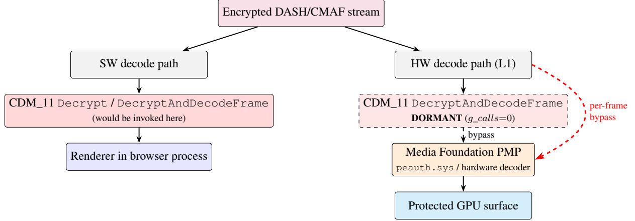
Figura 4: Hardware-decode dormancy. Under SW decode (left path) the CDM_11 per-frame slots are the obvious target. Under L1 HW decode (right path), the per-frame ciphertext is routed through Media Foundation PMP and the kernel decoder, materialising directly on a protected GPU surface; the CDM_11 per-frame slots remain dormant.
