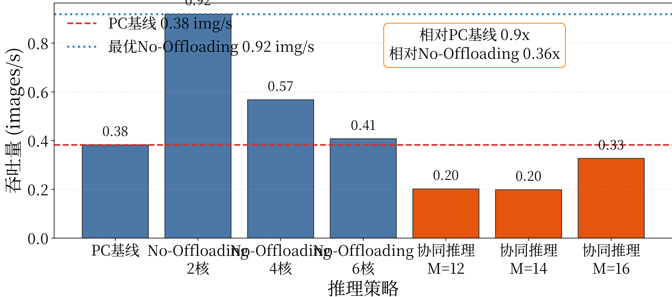
ResNet50 极端负载下真实协同推理性能
