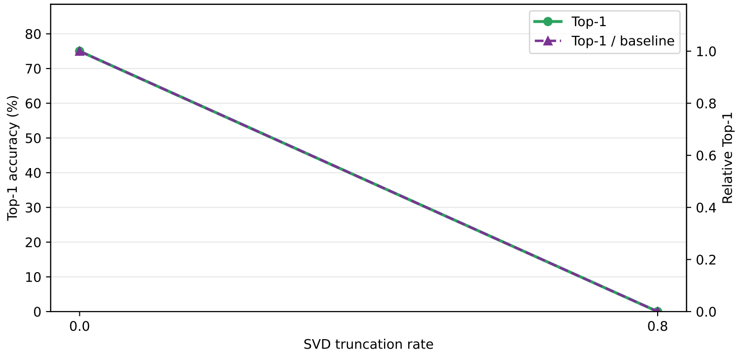
ResNet50 llama.cpp CPU SVD Top-1 on ImageNet-4
