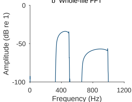
b Whole-file FFT
