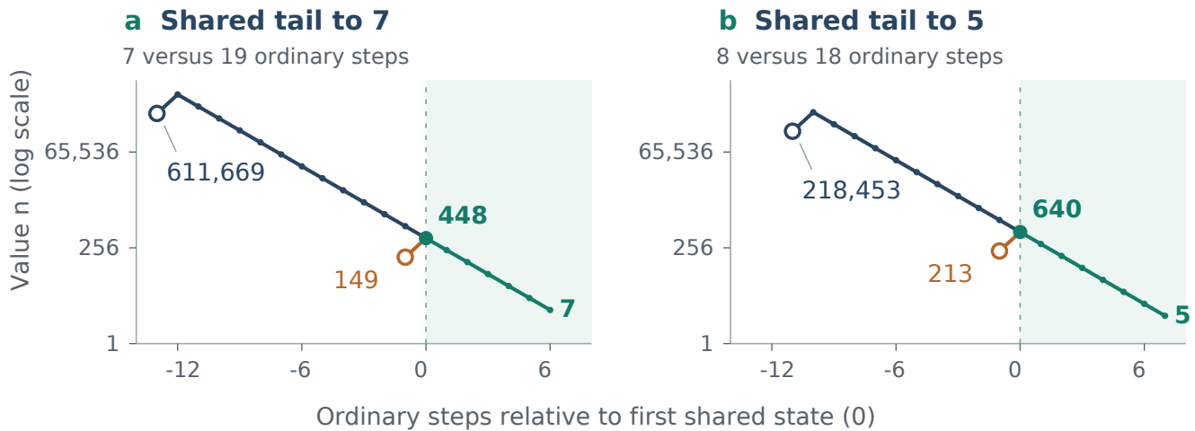
Figure 2. Distinct source histories join at 448 (a) and 640 (b); the identical subsequent states are drawn once in the shaded region. Time is aligned at the first shared state, not at the starts. Open circles mark sources. The current state cannot distinguish these histories. Exact archived fixtures; manuscript §7 and Appendix F .
