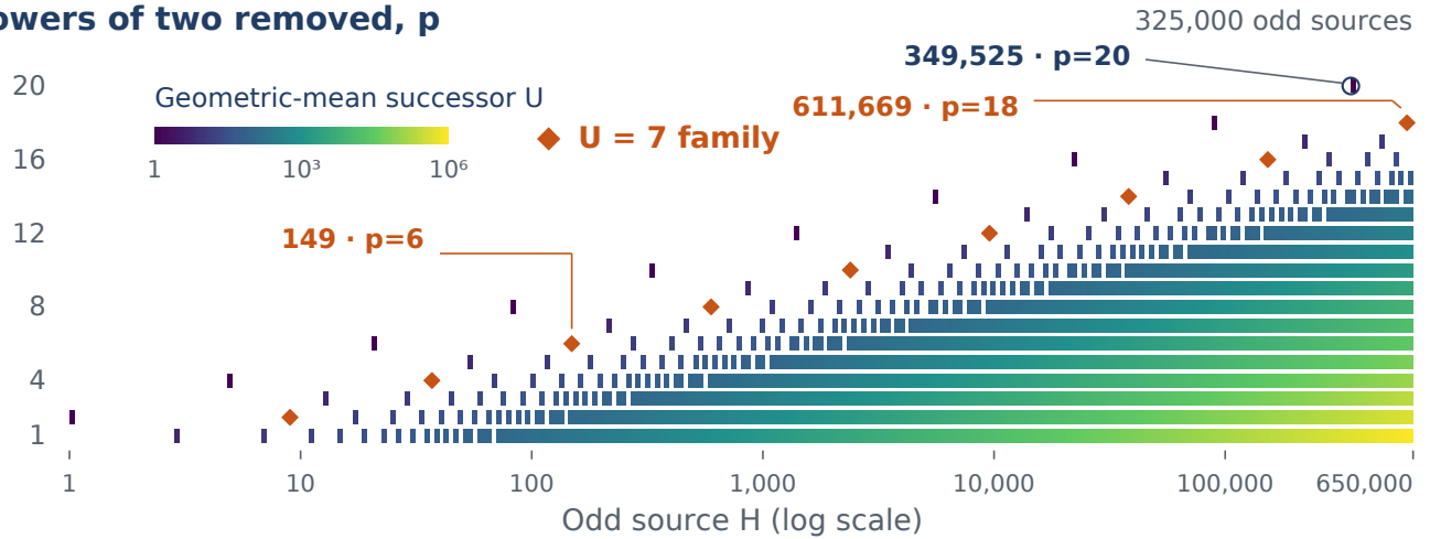
Figure 1. All 325,000 odd sources H \leq 649999 , with p = \nu_2(3H+1) . Color summarizes U in 280 logarithmic source bins; orange diamonds mark all nine U = 7 sources. The p = 20 point is included. This finite map is not the complete fiber .
