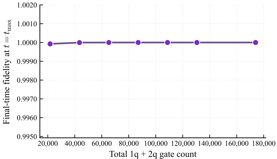
Harmonic fidelity vs total gate count
