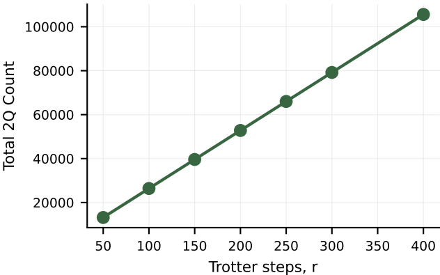
Harmonic oscillator CX count
