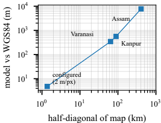
(b) flat-earth model error
