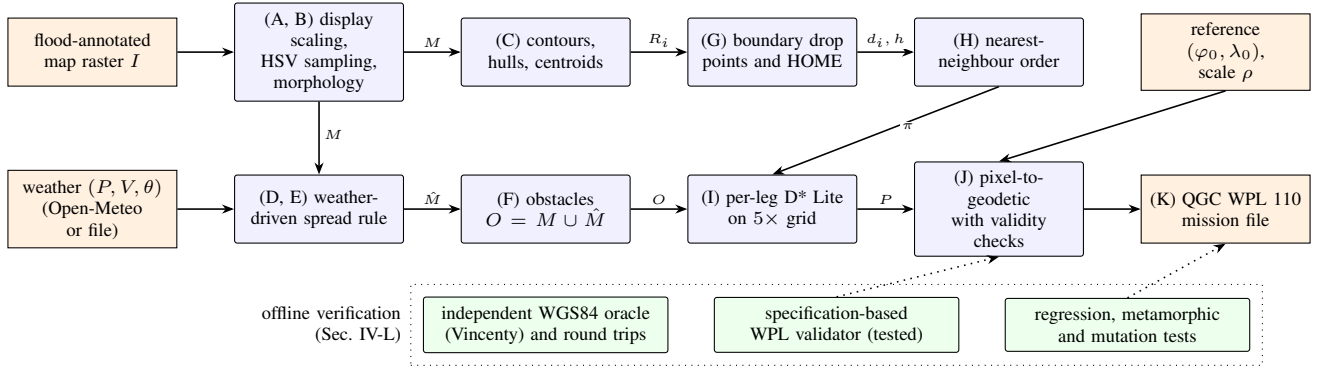
Fig. 1. Architecture of A.D.A.P.T. as implemented. Letters refer to the subsections of Section IV. Blue boxes are pipeline stages executed in this order by the entry point; orange boxes are inputs and the output. The dotted block is the offline verification layer, which is not part of the run-time pipeline. Colour sampling is the only interactive step.
