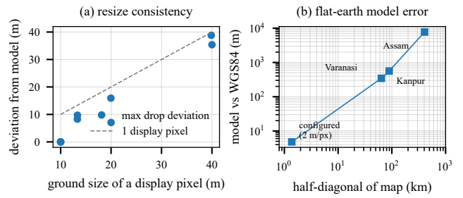
Fig. 9. (a) Maximum deviation of drop coordinates from the model across display widths, against the ground size of one display pixel. (b) Worst-case model error against WGS84 versus map half-diagonal: the configured 2 m/px setting and the landmark-estimated real extents of the three maps.
