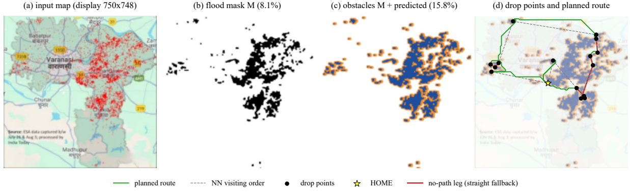
Fig. 3. Pipeline stages for the Varanasi map. (a) Input after display scaling (third-party map; see Data Availability). (b) Flood mask M . (c) Obstacles: M (blue) and predicted-only pixels \bar{M} \setminus M (orange). (d) Drop points, HOME, nearest-neighbour order (dashed), planned route (green) and the 8 no-path legs flown as straight segments (red).
