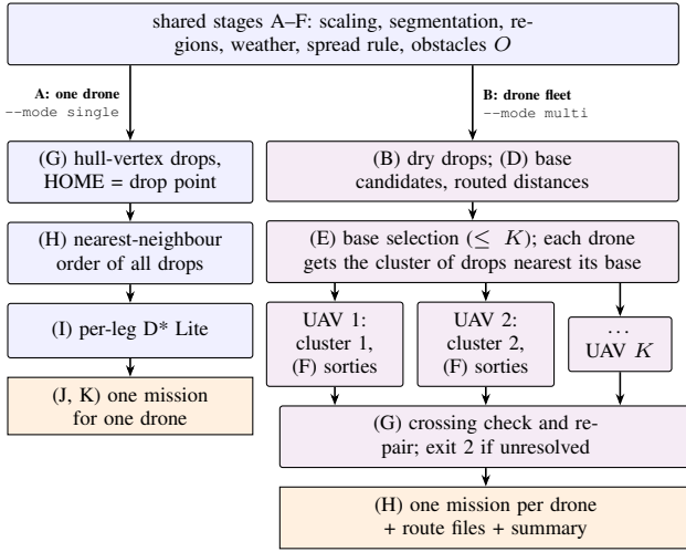
Fig. 2. The two planning approaches. Left, Approach A: one drone visits every drop point (single-UAV pipeline, Section IV). Right, Approach B: a fleet of up to K drones (multi-base mode, --max-bases K ; Section V, whose subsections the letters refer to). Each drone flies battery-limited sorties from its own base to the cluster of drop points nearest that base. The drones are planned independently and coordinated only by the pre-flight crossing check; K = 1 yields one drone.
