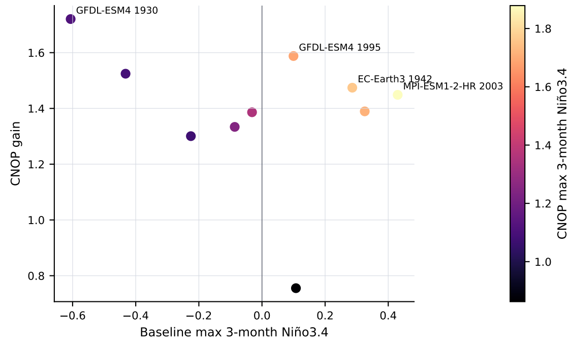
D Where CNOP amplification is largest
