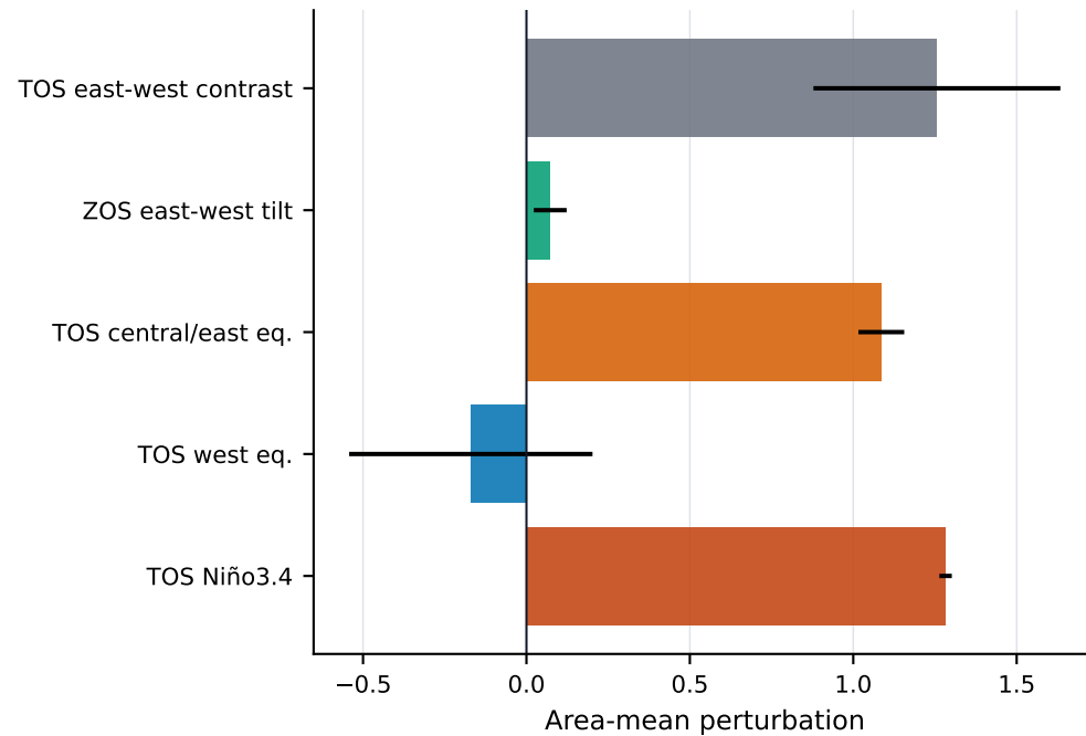
D Where CNOP amplification is largest
