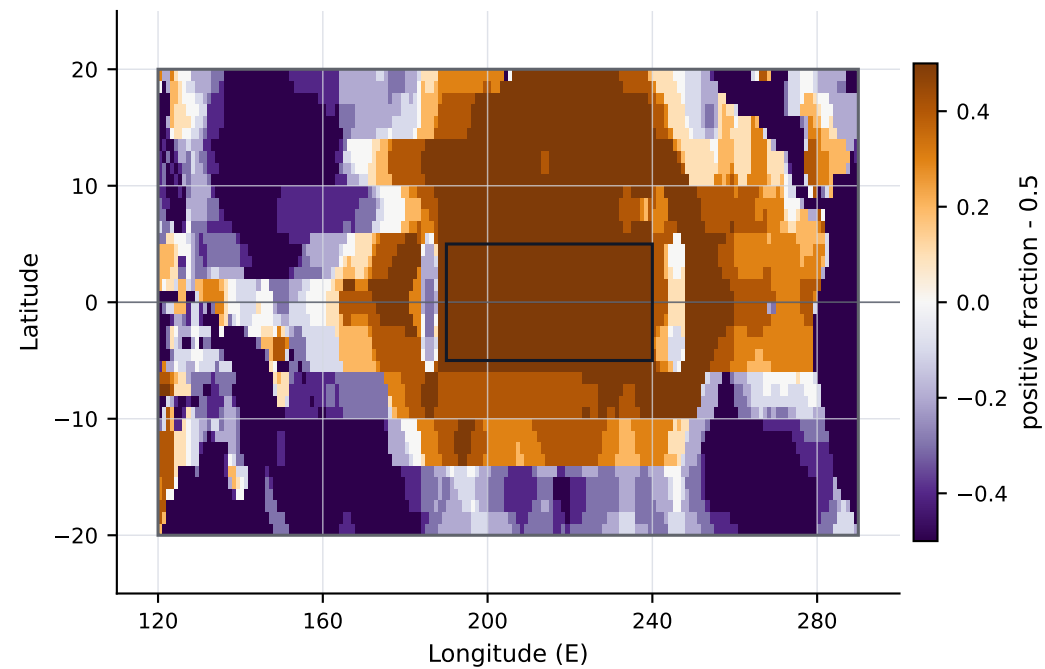
B TOS sign agreement across neutral cases
