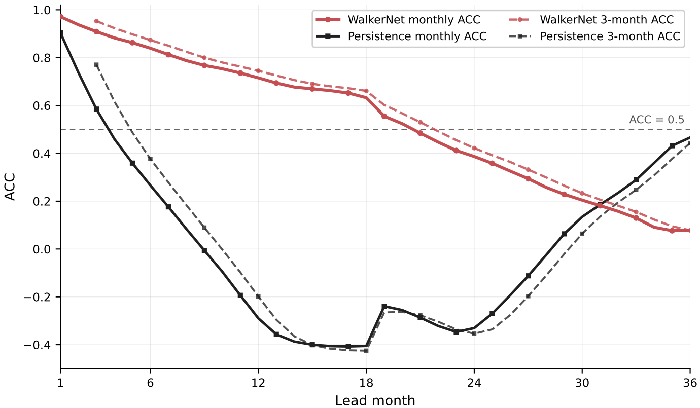
WalkerNet Niño3.4 forecast skill
