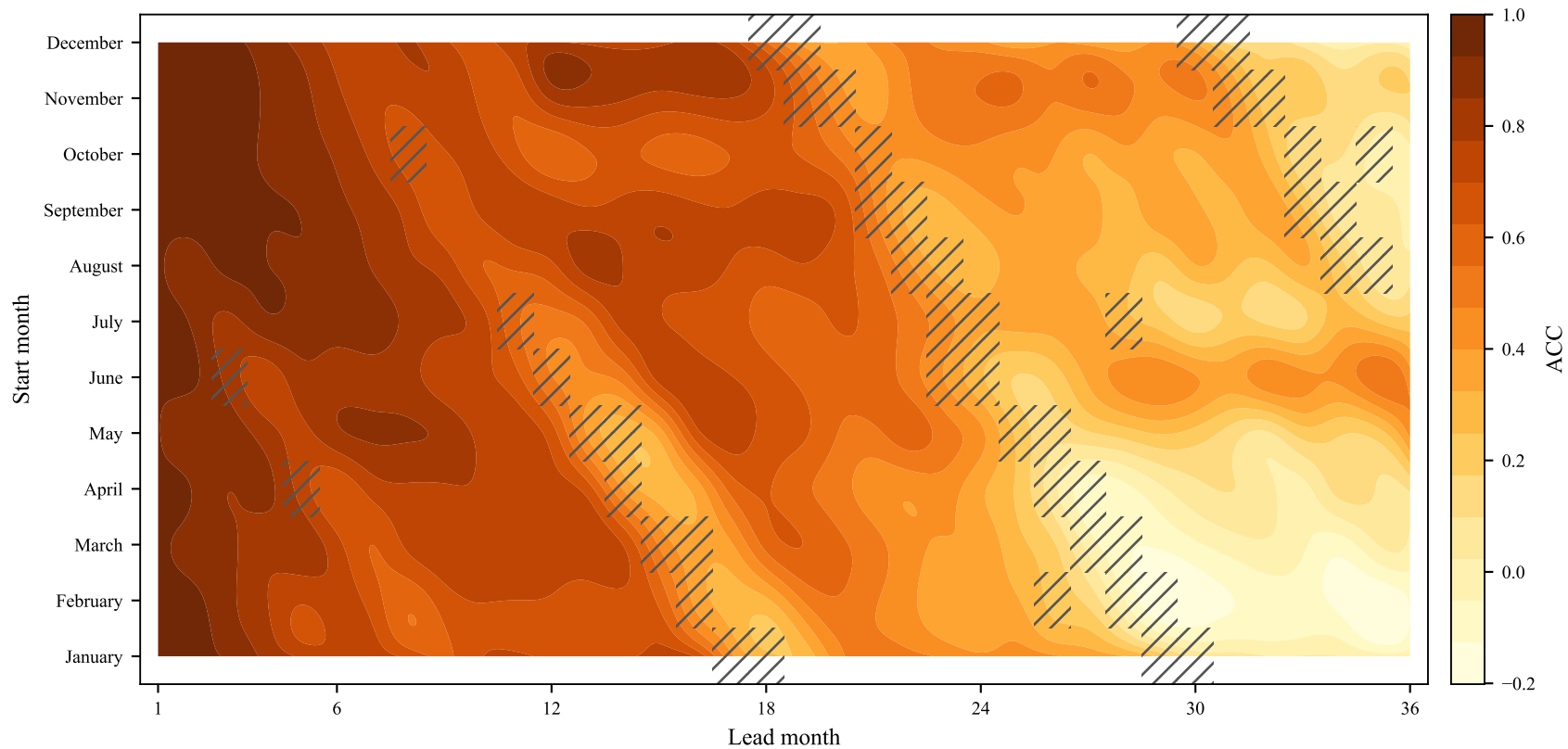
Nino3.4 ACC by forecast start month
