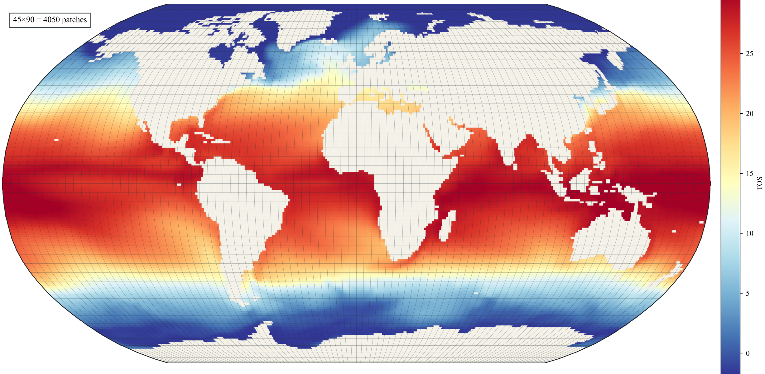
WalkerNet TOS training sample with 4^\circ \times 4^\circ Robinson patch grid (CESM2, time index 0)
