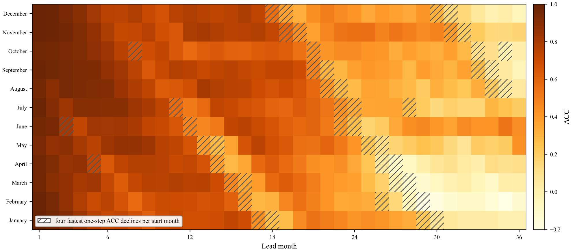
Nino3.4 ACC by forecast start month
