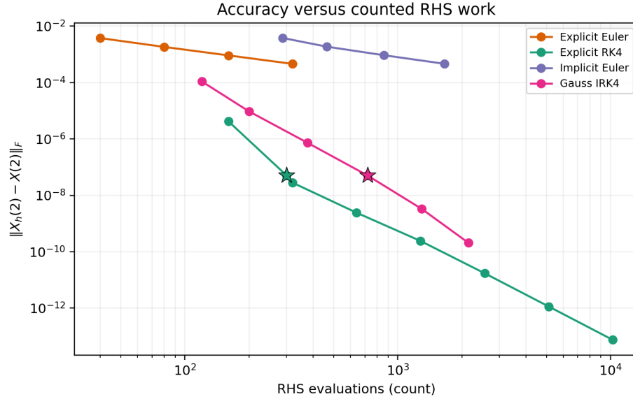
Figure 11: Terminal error versus counted right-hand-side evaluations. The highlighted RK4 and Gauss IRK4 runs have terminal errors differing by approximately 0.3%. The plotted work measure does not include Jacobian assembly, linear solves, or Python overhead.
