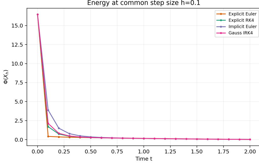
Figure 12: Sampled Lyapunov energy trajectories for the four methods on the common grid h = 0.1 . All sampled trajectories decrease in this experiment; this is an empirical observation rather than a general monotonicity theorem.
