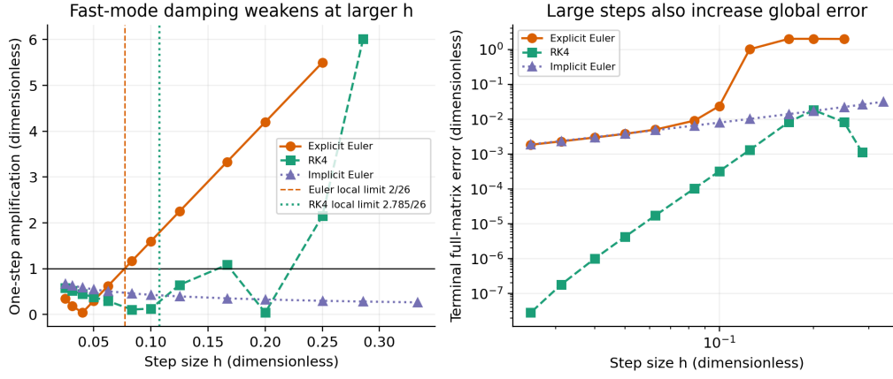
Figure 4: Left: one-step amplification of a fast-direction initial perturbation. Right: terminal error for completed runs on log-log axes. The labelled vertical lines show Euler and RK4 limits from the initial frozen Jacobian; they are local estimates, so the nonlinear sweep is needed to assess their relevance. Energy changes and failed-run statuses are in stability_sweep.csv .
