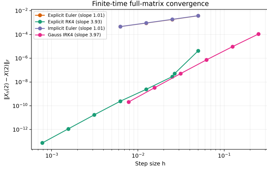
Figure 10: Terminal Frobenius-norm error versus step size for the four numerical methods. The fitted Gauss IRK4 slope on the refined grids is approximately 3.9674, consistent with fourth-order behaviour on the tested finite grids.
