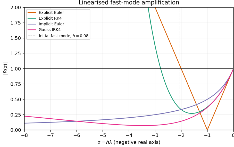
Figure 9: Comparison of the scalar stability amplification factors along the negative real axis. The dashed reference marks the initial frozen mode z = -26 \times 0.08 = -2.08 . The Gauss IRK4 curve illustrates its A-stability and its lack of L-stability.
