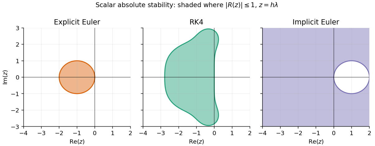
Figure 1: Absolute-stability sets |R(z)| \leq 1 computed from the amplification functions. The three panels show Explicit Euler, RK4, and Implicit Euler, respectively. The coloured masks visualize the analytical regions in the dimensionless z = h\lambda plane; they do not by themselves establish nonlinear stability.
