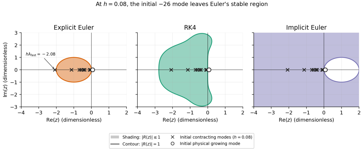
Figure 1: Absolute-stability sets |R(z)| \leq 1 computed from the amplification functions. The three panels show Explicit Euler, RK4, and Implicit Euler, respectively. The coloured masks visualize the analytical regions in the dimensionless z = h\lambda plane. Crosses locate the eight contracting eigenmodes of the initial Jacobian at h = 0.08 ; the open circle marks the physically growing +0.88 mode. These frozen-spectrum markers do not by themselves establish nonlinear stability.
