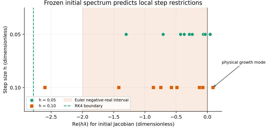
Figure 2: The initial Topic 5 Jacobian spectrum scaled by h = 0.05 and h = 0.10 . The two categorical rows distinguish step sizes; their vertical positions do not represent imaginary parts. The +0.88 mode reflects physical growth of the initially small singular value, while h = 0.10 moves the fastest negative mode past Euler’s -2 boundary.
