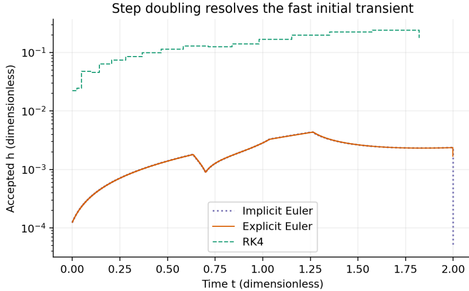
Figure 5: Accepted step length versus dimensionless time. Step doubling reduces the step during the rapid initial transient; the accepted-step data and estimated local error are in adaptive_steps.csv .
