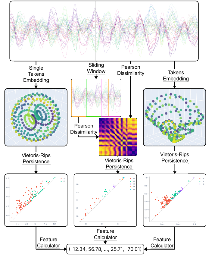
Fig. 3. The scheme of the algorithm for extracting the topological features from the EEG.
