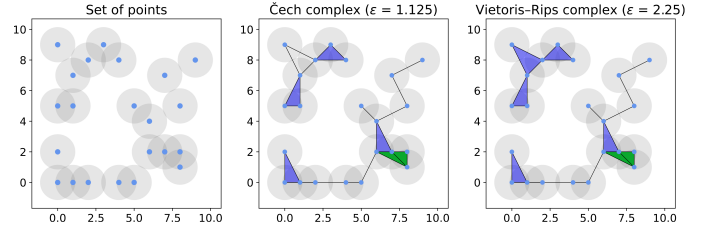
Fig. 2. A synthetic point cloud with its Čech and Vietoris–Rips complexes for some values of the filtration parameter.
