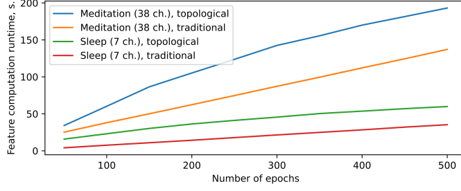
Fig. 5 The running time of calculating traditional and topological features for two types of data, depending on the number of epochs. Each point is an average of 25 measurements. The 95% confidence intervals for each entry do not exceed 1% of their absolute value
