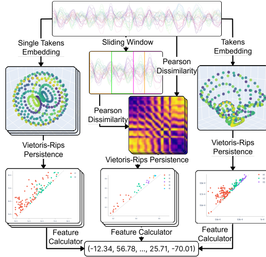
Fig. 1 The algorithm for extracting topological features from the EEG
