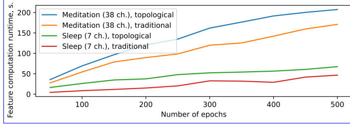
Fig. 7 The running time of calculating traditional and topological features for two types of data, depending on the number of epochs. Each point is an average of 25 measurements. The 95% confidence intervals for each entry do not exceed 1% of their absolute value
