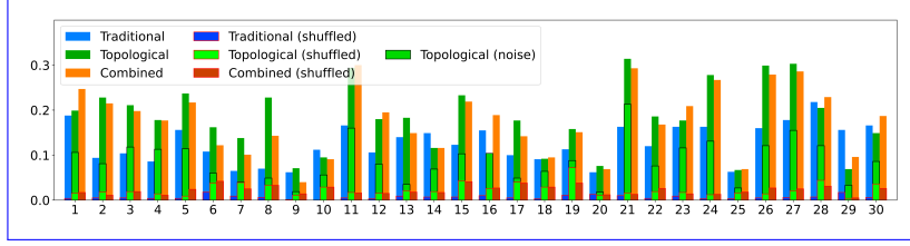
Fig. 5 The adapted silhouette scores of the resulting boundaries deduced by SDA using three types of features for the original and shuffled recordings of 30 subjects
