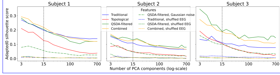
Fig. 3 Adapted silhouette scores of results for subjects 1 – 3 using different sets of features with a varying number of PCA components
