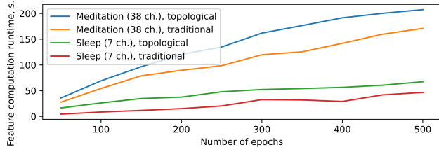
Fig. 8 The running Running time in seconds for calculating traditional and topological features from EEG with varying numbers of epochs. Each point is an average of 25 measurements on a standard 8-core Intel Ice Lake VM with 16 GB of RAM. The 95% confidence intervals for each entry do not exceed 1% of their value
