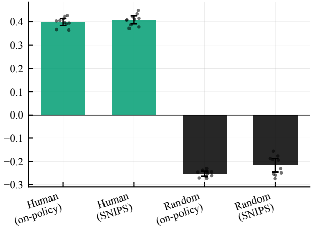
Mean reward per decision
