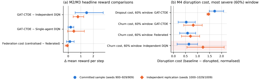
Fig. 7 Every headline paired comparison in this paper, committed sample (seeds 900–929/909) against the independent replication sample (seeds 1000–1029/1009), recomputed from raw logs for both. (a) M2/M3 reward comparisons. (b) M4 disruption cost at the most severe (60%) window. The bottom row of (b), independent DQN’s churn cost, is the one comparison whose two samples visibly disagree on more than point-estimate noise – the finding retracted in Section 9-D.
