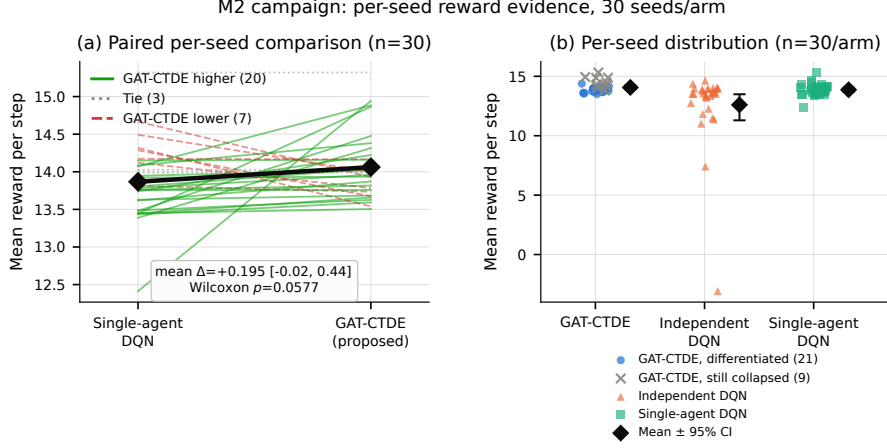
Fig. 3 30-seed campaign, per-seed evidence for mean reward per step, the correctness-aware metric (Section 5.6). (a) Paired per-seed comparison against single-agent DQN: each line is one seed, coloured by whether GAT-CTDE scored higher (green, 20), tied (grey, 3), or lower (red, 7) than the baseline on that seed – the same paired unit the Wilcoxon test is computed over, and the source of this figure’s borderline p = 0.0577 . (b) Full per-seed distribution for all three arms; GAT-CTDE is split into seeds that learned genuine differentiated shedding (blue, 21) versus seeds still stuck at the always-accept collapse (grey \times , 9) – shown without claiming the split predicts reward, since several still-collapsed seeds score among the arm’s highest (always accepting never pays the reject cost).
