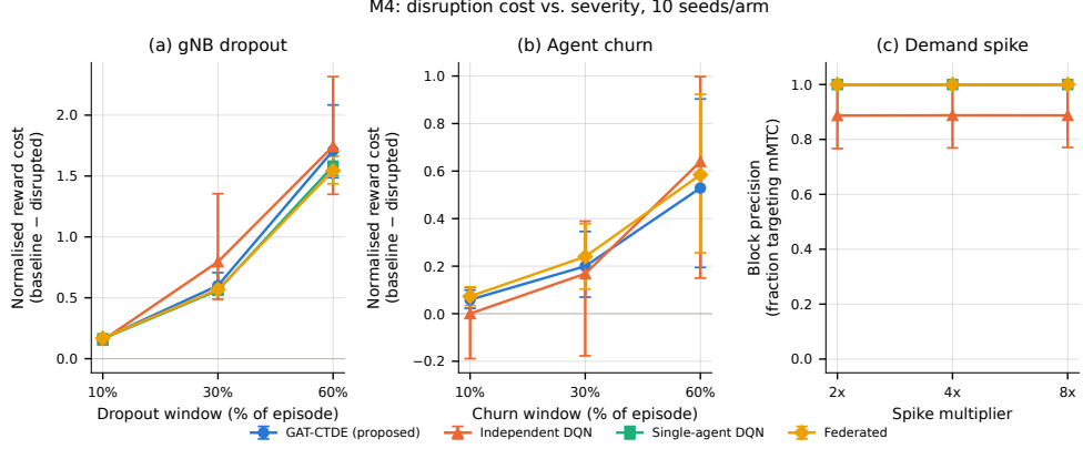
Fig. 5 M4 disruption campaign, 10 seeds/arm. (a)-(b) Normalised reward cost (baseline – disrupted) vs. severity for dropout and agent churn – every arm, every severity, shows a real cost that accelerates with severity rather than growing linearly. (c) Block precision vs. demand-spike multiplier: flat and near-ceiling for every arm, unlike (a)-(b) – spike does not threshold on the metric that matters.
