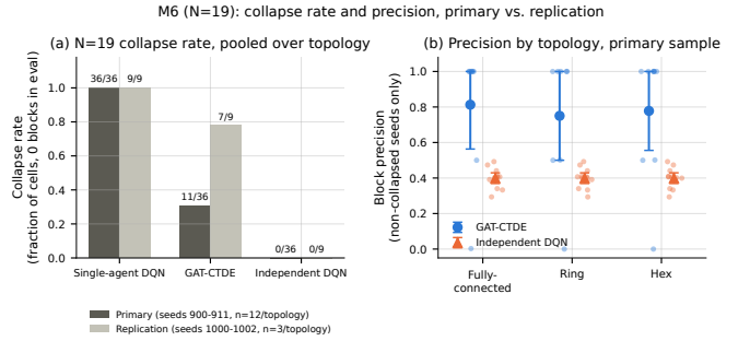
Fig. 8. N = 19 cluster, per-seed evidence. (a) Collapse rate (fraction of eval runs with zero blocks), pooled across all three topologies, primary sample (seeds 900–911) against the independent replication sample (1000–1002) – single-agent DQN collapses totally in both; GAT-CTDE’s own rate is markedly higher in the replication sample. (b) Block precision by topology, primary sample, non-collapsed seeds only (single-agent DQN has none to show): GAT-CTDE’s non-collapsed seeds are mostly near-ceiling but with a low-precision seed at every topology, while independent DQN sits in a narrow, mediocre band, identical across topologies as expected for an arm that never consumes adjacency.
