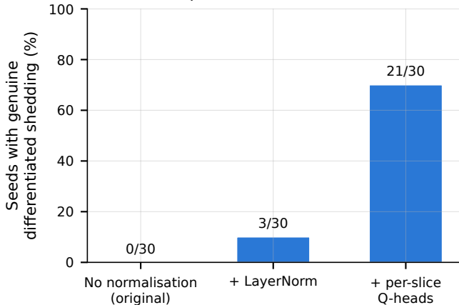
GAT-CTDE collapse reduction across encoder fixes
